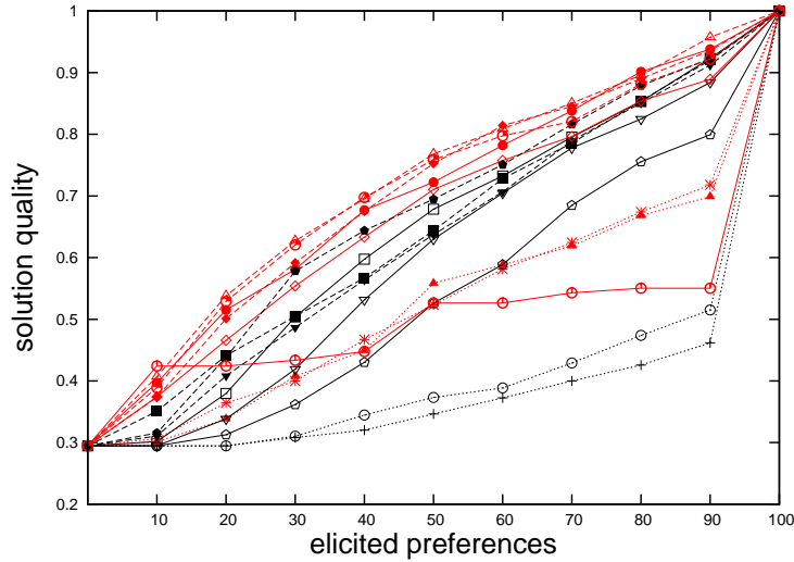
Figure 7: Incomplete fuzzy CSPs: solution quality.
