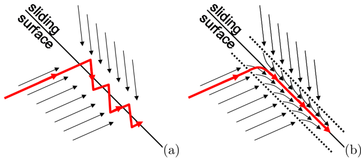
Figure 6: The left figure illustrates chattering at the sliding surface. The right figure illustrates the effect of a boundary layer.
