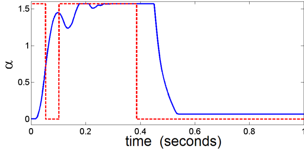
Figure 5: The throttle angle (solid) in response to an input (dashed) that changes between a wide open throttle, and a fully closed throttle.
