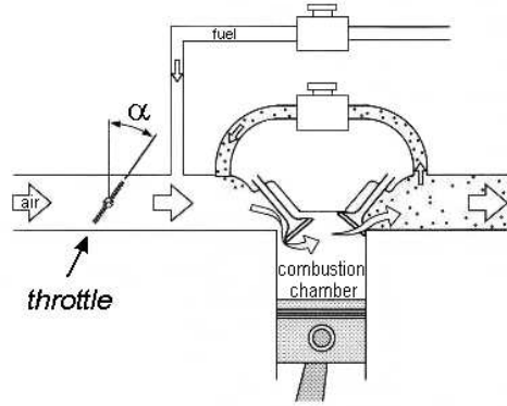
Figure 2: The angle of the throttle plate determines the air flow, and indirectly the engine speed.
