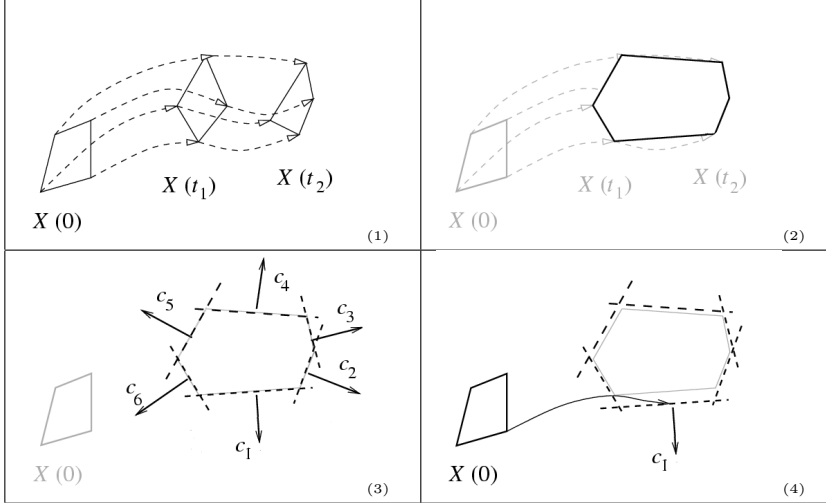
Figure 1: Steps in the flowpipe approximation are (1) simulating the vertices, (2) enclosing the simulation points in a polyhedron, (3) determining the normals and (4) increasing the size of the polyhedron, until it contains the complete segment.
