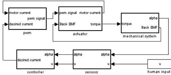
Figure 3: An automotive throttle control system.
