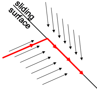
Figure 4: Illustration of the concept of sliding-mode control.
