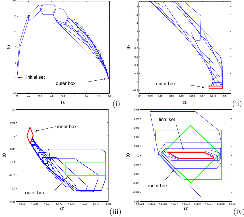
Figure 7: Figure (i) and (ii) depict the flowpipe approximation for the transient phase. Figure (ii) is a close up of Figure (i). Figure (iii) depicts the flowpipe approximation in the neighborhood of the steady-state value. Finally, Figure (iv) shows that the states that start in the inner box will eventually return to this set. Note that these figures show projections of the flowpipe segments onto throttle angle \alpha and angular velocity \omega .
